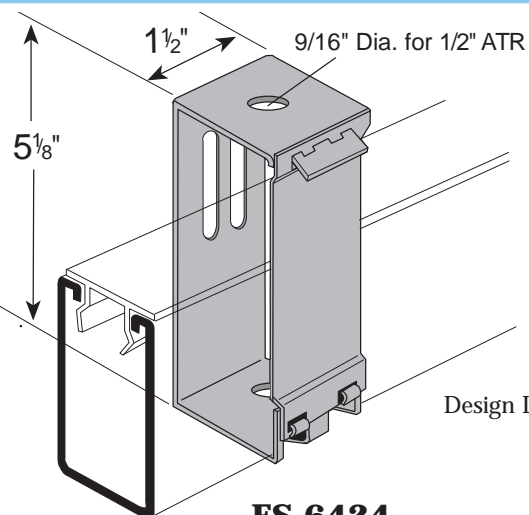
FS-6424 DEEP CHANNEL HANGER
